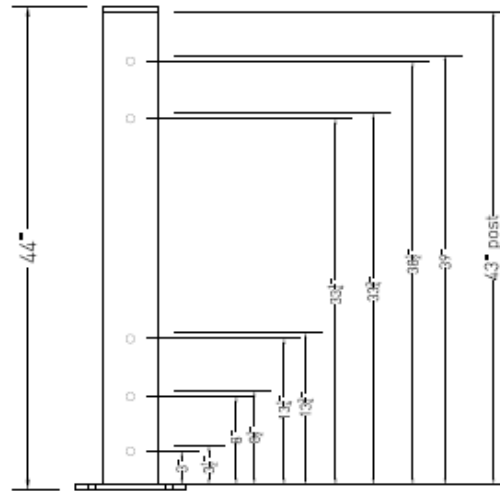
DOUBLE RAIL POST
