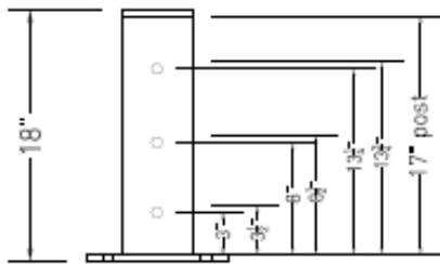
SINGLE RAIL POST
